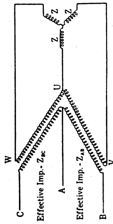
FIG. 4—OPEN DELTA OR V CONNECTION.
