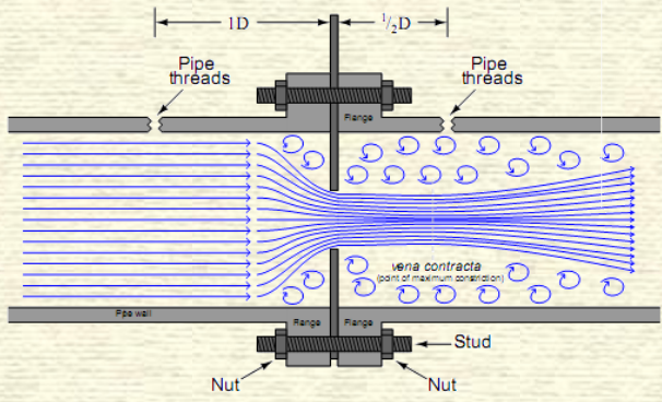
Radius taps
