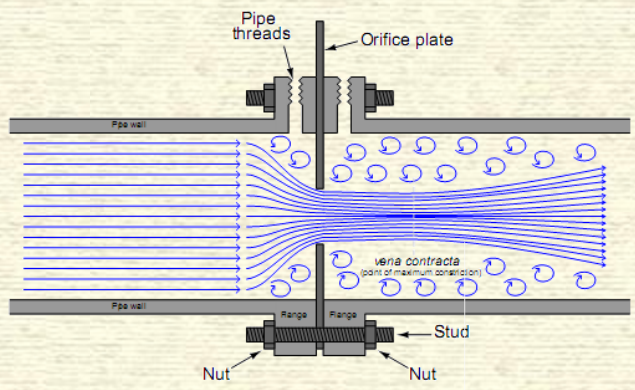
Flange taps
