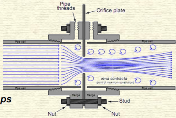
Corner taps
